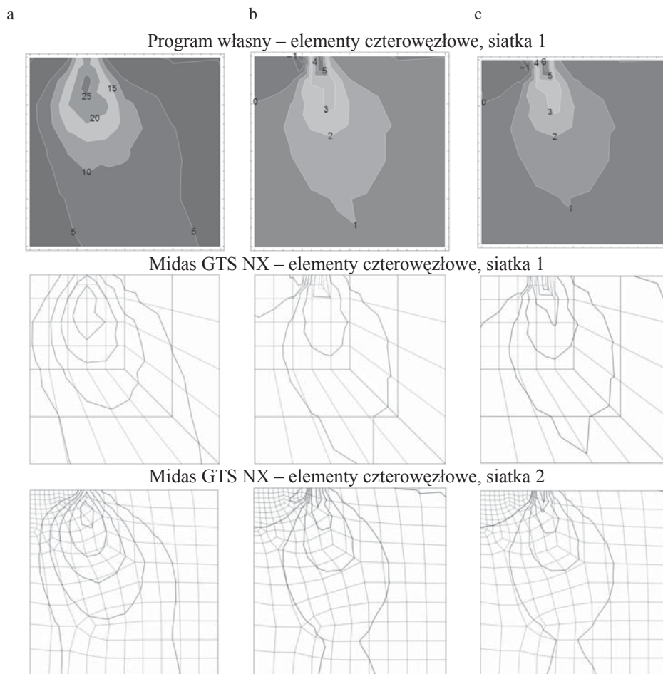
Fig. 7. Ground surface settlements: a – own calculation for 4 node elements, b – calculation for 8-node elements [Potts and Zdravkovic 1999]
