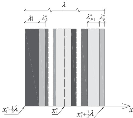
Fig. 1. The scheme of one of the layer in multicomponent multilayered composite with functional gradation of effective material properties
